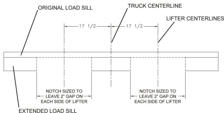
TOP VIEW OF TRUCK LOAD SILL
