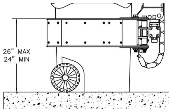
Gripper Arm mounting height
